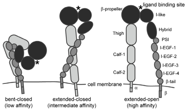
Figure 1. Integrins exhibit three distinct conformations correlated with binding affinity. Headpiece domains are depicted in black. In the low affinity conformation, the integrin leg domains are bent and the headpiece is closed. In the intermediate affinity conformation, the leg domains are extended and the headpiece is closed. In the high affinity conformation the leg domains are extended, and the headpiece is open. doi:10.1371/journal.pone.0015746.g001
